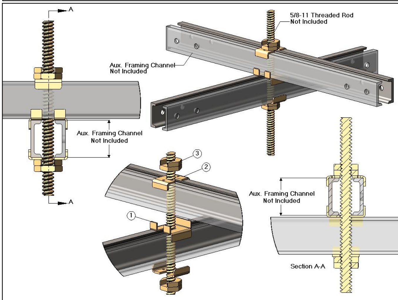
FCA326 - Aux. Framing Channel Crossover Slotted Clip Kit
